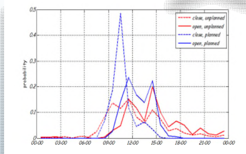
TIME OF VALVE OPERATION DURING PLANNED AND UNPLANNED REPAIR
