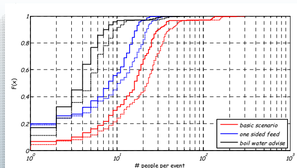
EFFECT OF A ONE-SIDED FEED OR BOIL WATER ADVISORY ON THE ESTIMATED NUMBER OF PEOPLE INFECTED
