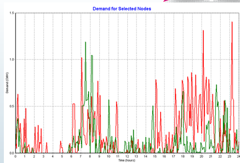
SIMDEUM DEMAND PATTERNS
