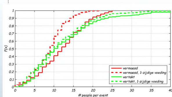
EFFECT OF THE NETWORK LAYOUT ON NUMBER OF PEOPLE INFECTED
