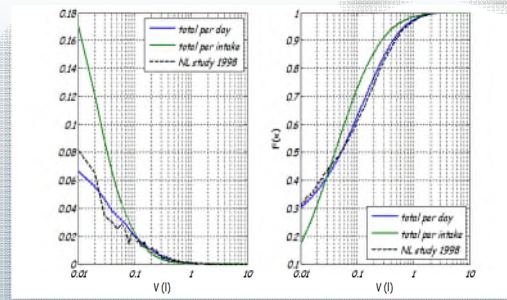
DAILY VOLUME OF TAP WATER INGESTED
