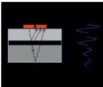
Afb. 2: Principeschets radarmeting.
