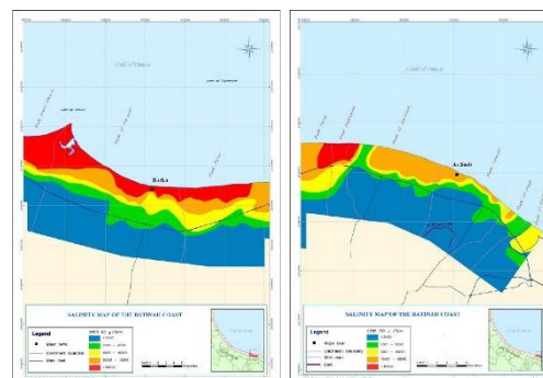
Figure 2: Maps of groundwater salinization in the coastal plain of Al Batinah, Oman 20
