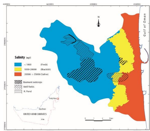
Figure 10: Map of Groundwater Salinity in Fujeirah, UAE 34
