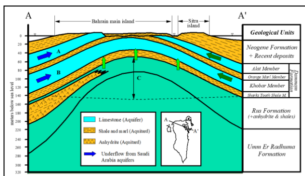
Figure 5: Hydrogeological West-East cross-section of Bahrain with three aquifers: A - Alat member, Damman formation, B -Khobar member, Damman formation, C - Rus-UER aquifer system 26
