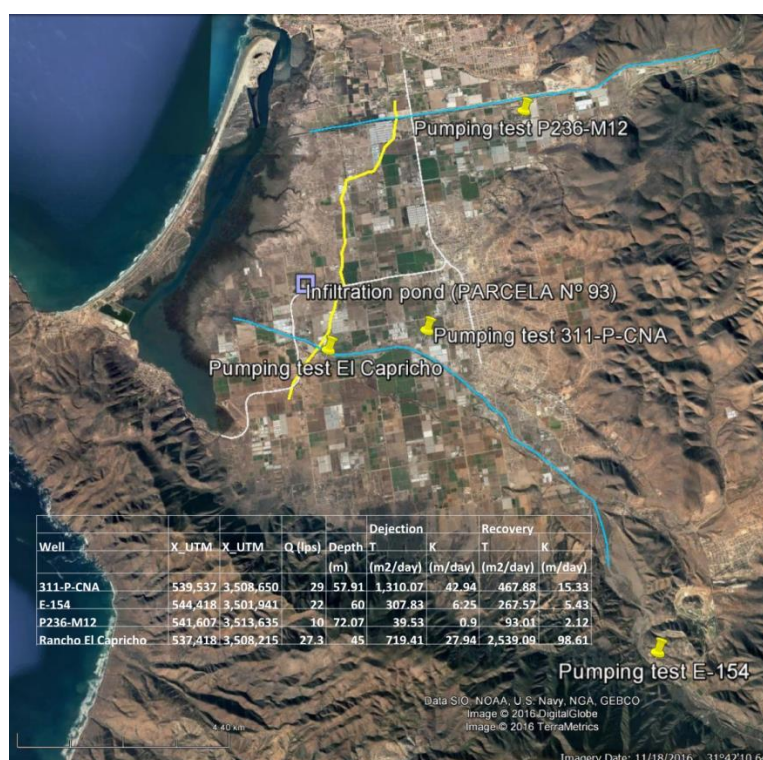
Figure 11 Location of the pumping tests performed in the Maneadero Aquifer (yellow pins) and of the salt water infiltration measured through geophysical methods ((LUJÁN and Romo 2010))
