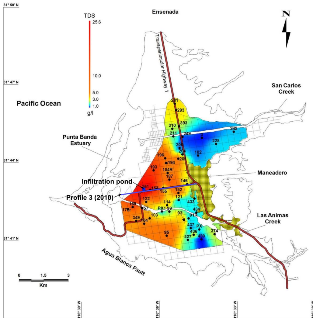
Figure 13 TDS distribution in 2011 based on geophysical studies by CICESE. The blue dot indicates the location of the infiltration pond and the blue line the location of the third geophysical profile performed by (LUJÁN and Romo 2010). Modified after (Daesslé, Pérez-Flores et al. 2014)
