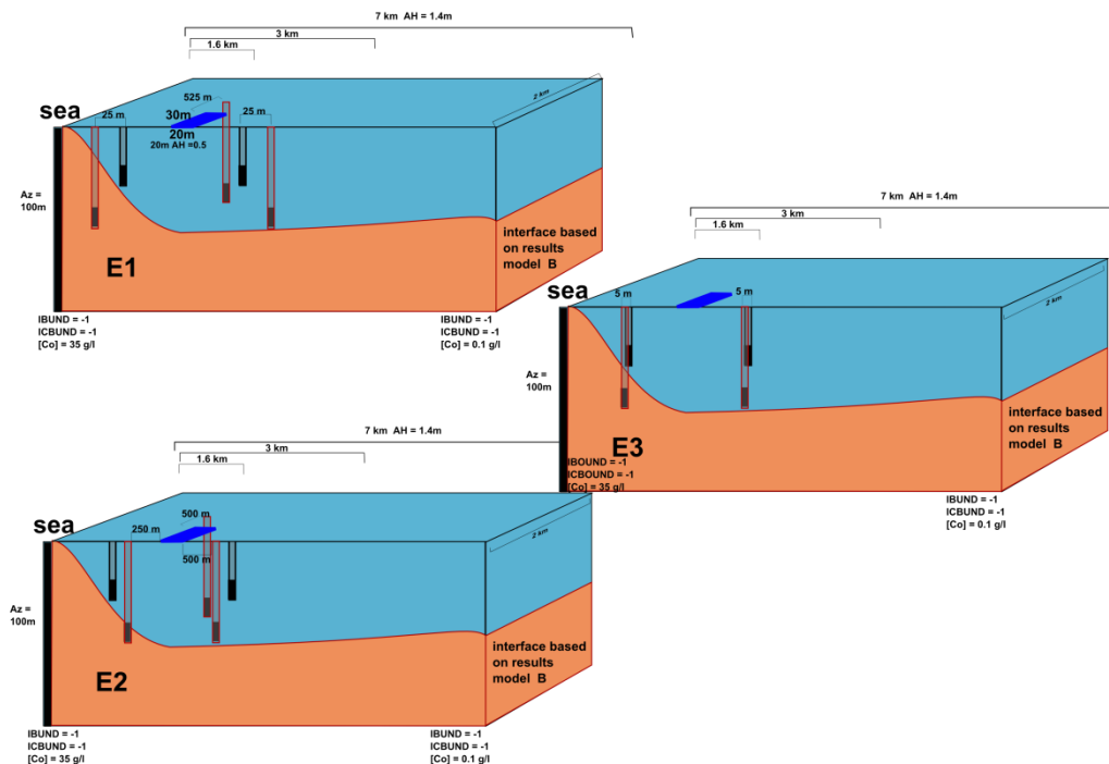
Figure16. Scenarios run with different Freshkeeper configurations related to the existing wells. The blue rectangle represents the infiltration pond, the orange part of the aquifer the brackish groundwater and the blue the expected fresh groundwater.
