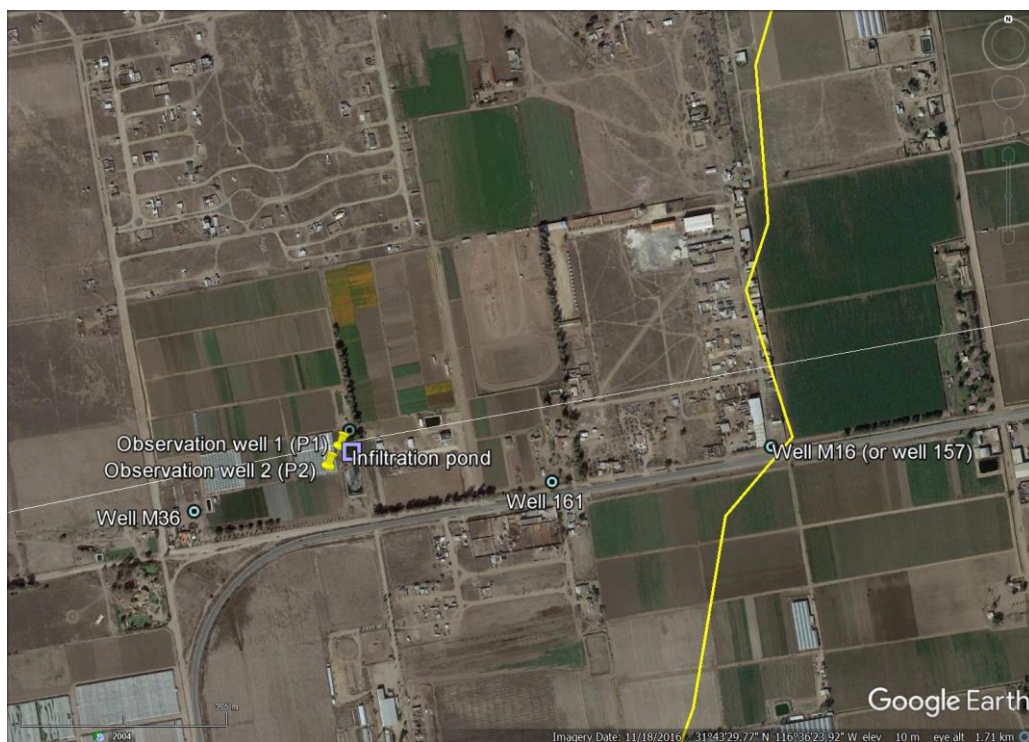
Figure 14 Location of the pumping and observation wells closest to the infiltration pond. The yellow line indicates the extension of the sea-water intrusion
