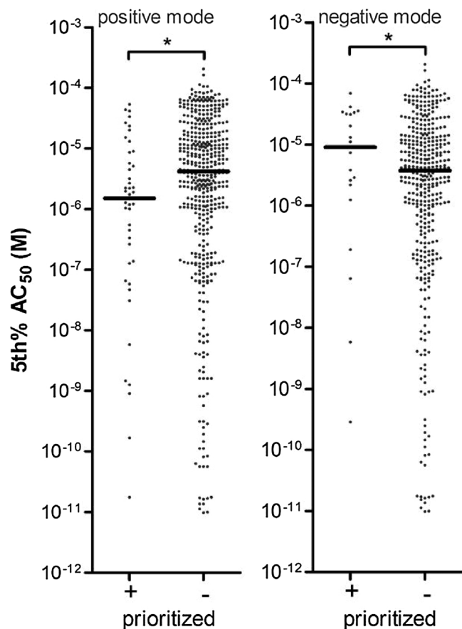
Fig. 3. Comparison of toxicity (5th percentile AC_{50} values) of suspects prioritized (+) or not (-) based on their semi-quantitative concentrations, detected in positive (left) or negative (right) ionization mode. Dots represent individual 5th percentile AC_{50} values, bars indicate the median.
