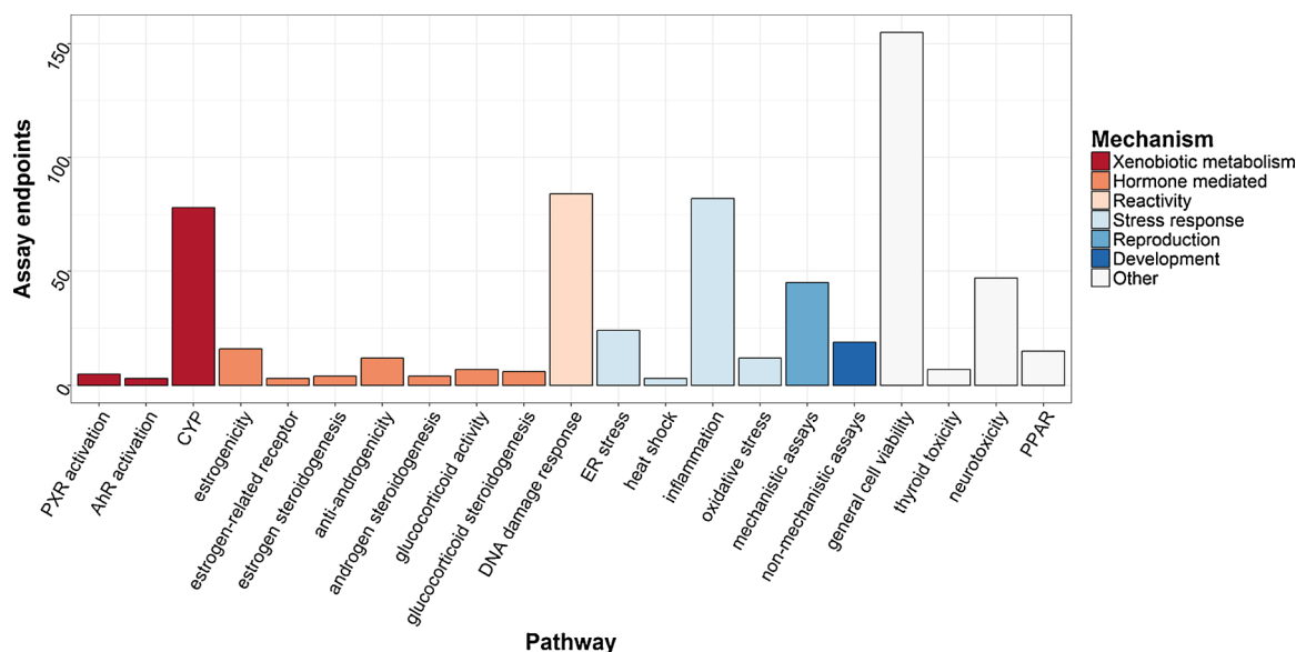
Fig. 1. Presence of water relevant mechanisms and related pathways in ToxCast database.
