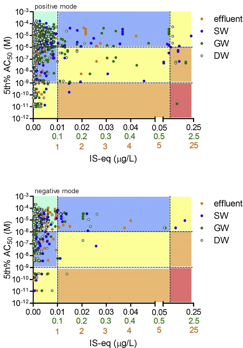
Fig. 4. Suspects detected in sewage treatment plant effluent (orange dots), surface water (SW, blue dots), groundwater (GW, green dots) and drinking water (DW, white dots) are plotted according to their toxicity (5th percentile AC 50 ) and exposure (ISeq, black data for GW/DW, green for SW, orange for effluent). The vertical dashed lines indicate the exposure threshold and 10x the threshold, the horizontal lines divide the 5th percentile values into three arbitrary potency classes of toxicity. Suspects detected in positive and negative ionization mode, respectively, are shown in the upper and lower panel.
