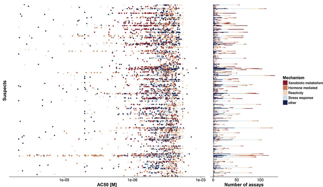
Fig. 2. AC_{50} values from water relevant ToxCast assay endpoints for detected suspect chemicals (left), and number of assays per mechanism (right) are shown.
