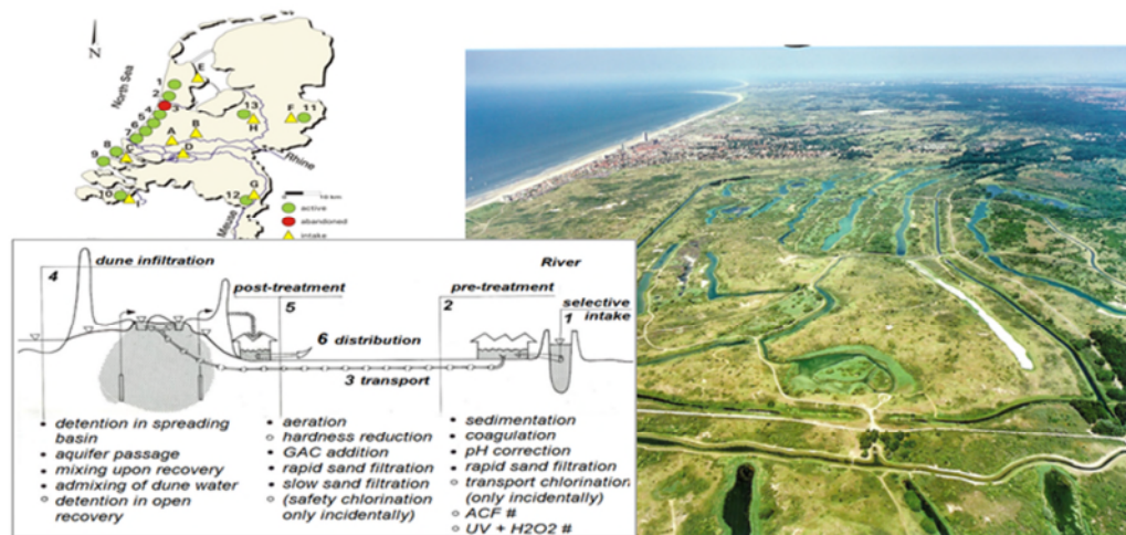
FIGURE 6-4. Basin artificial recharge in the Netherlands since 1940, in the period 2010-2014 producing on 12 sites ~200 Mm 3 /a (~16% of national drinking water supply). Figures from Stuyfzand (in prep), photo showing the Amsterdam dune catchment area from MAR calendar.
