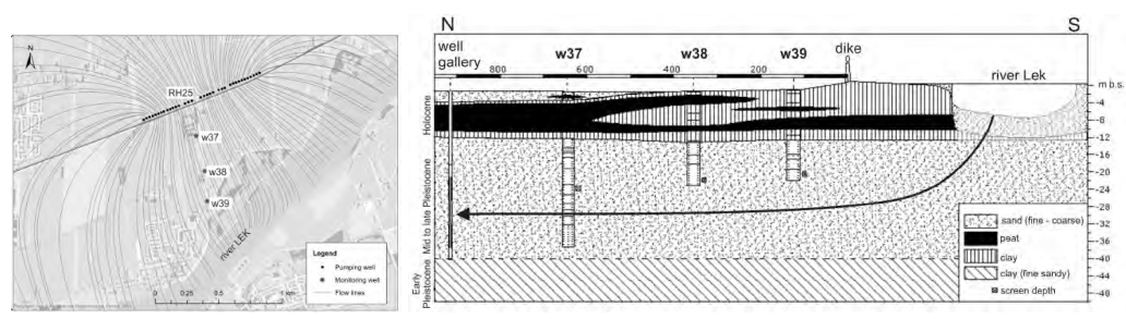
Figure 6-11. Hydrogeological conditions and position of the monitoring wells along transect Rodenhuis (modified from Segers (2006)). The arrow indicates the hypothetical groundwater flow.
