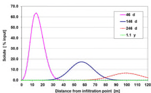
FIGURE 6-20. TRANSATOMIC predicted propagation of a dimethomorph pulse of 28 days through an anoxic homogeneous sandy aquifer towards a well at 120 m distance.
