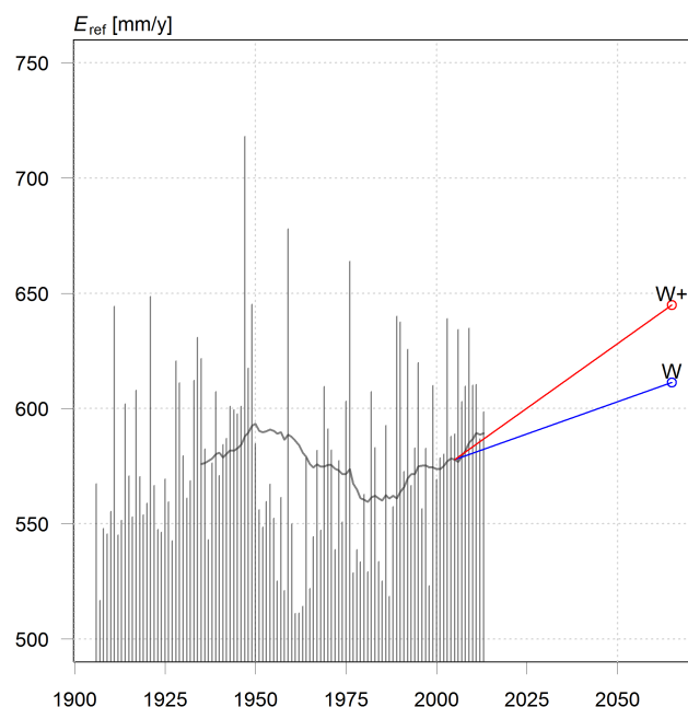
Figure 1. Yearly and 30-year moving average E_{\text{ref}} according to Penman–Monteith for De Bilt, the Netherlands, and projected E_{\text{ref}} values for the period 2036–2065. Projections are based on national climate scenarios (Van den Hurk et al., 2006) developed by the Royal Netherlands Meteorological Institute (KNMI). Two of the scenarios have been found to be most likely (Klein Tank and Lenderink, 2009) and are presented here: scenario W (blue line) and W+ (red line). Both comprise a +2 K global temperature increase, but with, respectively, unchanged and changed (+) air circulation patterns in summer and winter. The scenarios were used to transfer the climatic conditions of 1976–2005 to the period 2036–2065 (Van den Hurk et al., 2006).
