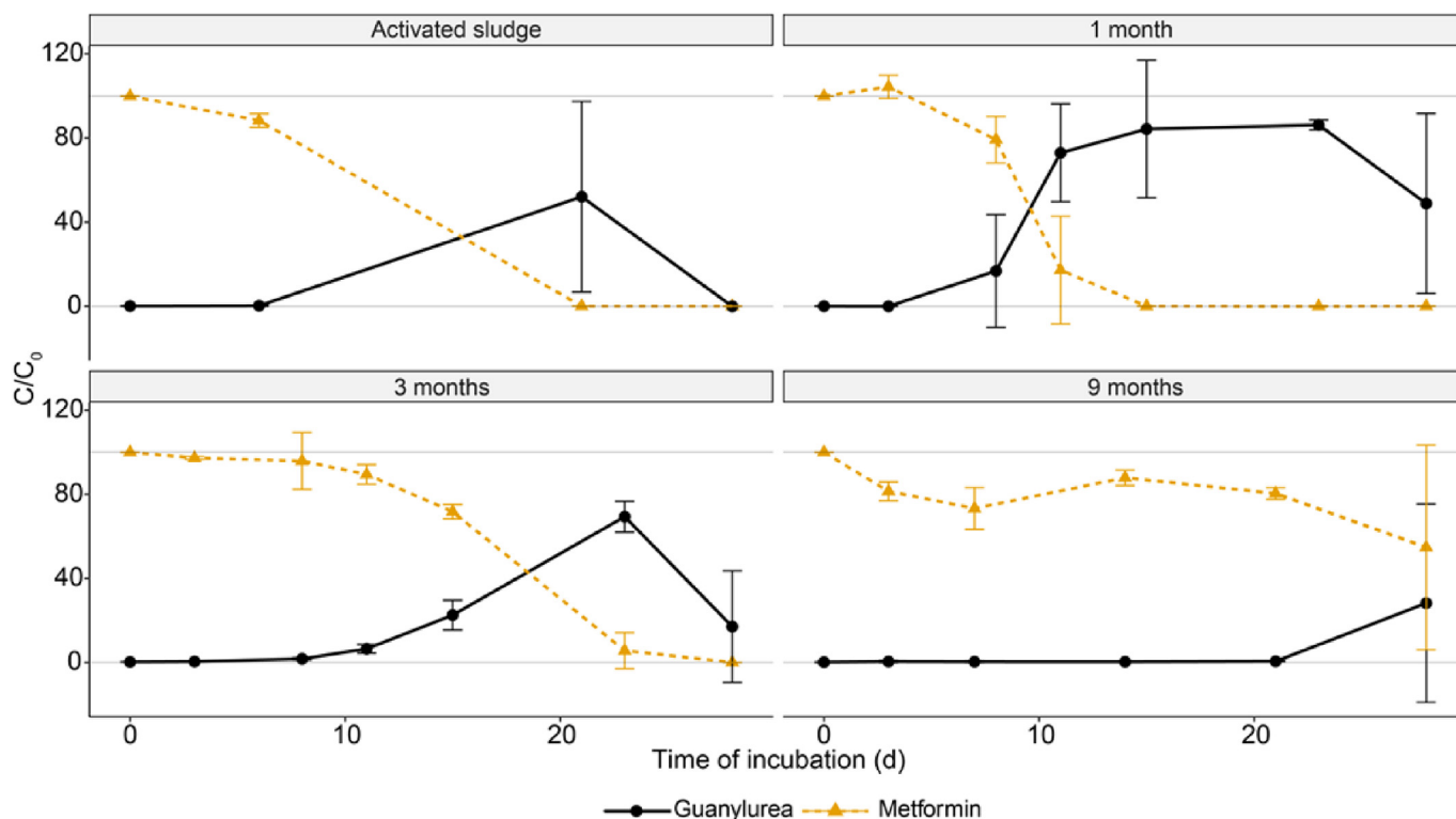
Fig. 2. Transformation of metformin to guanylyurea. Metformin degradation (%) is based on the measured concentration in sample divided by the original measure concentration ( C/C_0 ). Guanylyurea percentage (%) is based on the theoretical maximal transformation of metformin to guanylyurea, at the original measured concentration of metformin.
