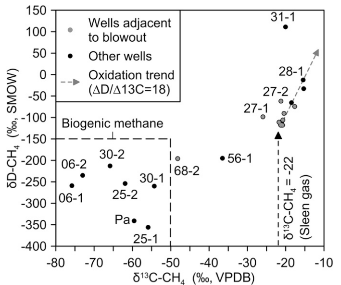
Fig. 5. \delta^{13}C-CH_4 vs. \delta D-CH_4 of analyzed groundwater wells. The gray arrow represents the calculated (according to ref. 30) isotopic enrichment due to AOM with \epsilon_C = 3 and \epsilon_D = 54 ( \Delta D/\Delta^{13}C = 18 ). In the absence of \delta D-CH_4 analyses from the Sleen gas field, the black arrow shows the \delta^{13}C-CH_4 of Sleen gas. SMOW, Standard Mean Ocean Water; VPDB, Vienna Pee Dee Belemnite.
