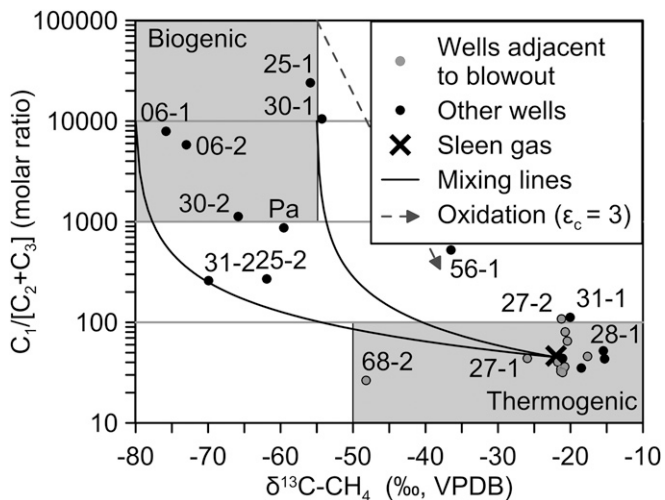
Fig. 4. C_1/(C_2 + C_3) vs. \delta^{13}C-CH_4 of analyzed groundwater wells. Mixing lines are between a thermogenic end member (average value of the three available samples from the Sleen gas field) and two possible biogenic end members [ C_1/(C_2 + C_3) of 10,000 and \delta^{13}C of -80\% and -55\% ]. Oxidation is calculated according to equation 15 of ref. 30. VPDB, Vienna Pee Dee Belemnite.
