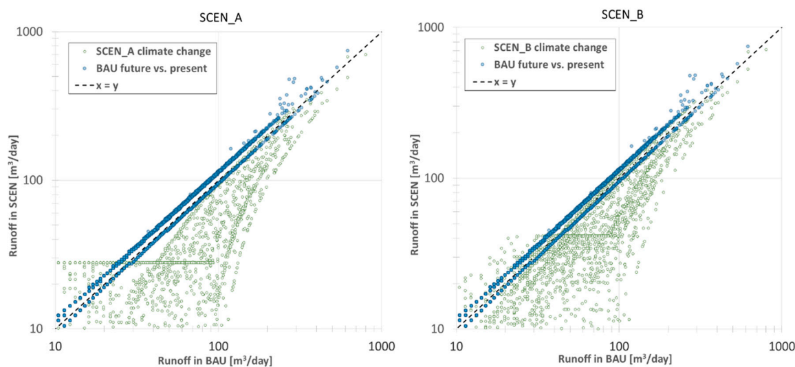
Figure 11. Event-based runoff reduction for a future reality and for both design options.
