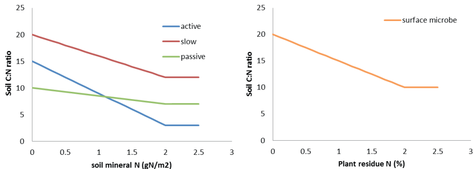
FIGURE 6 RELATION BETWEEN C:N RATIO AND SOIL MINERAL N (LEFT) AND PLANT RESIDUE N (RIGHT)
