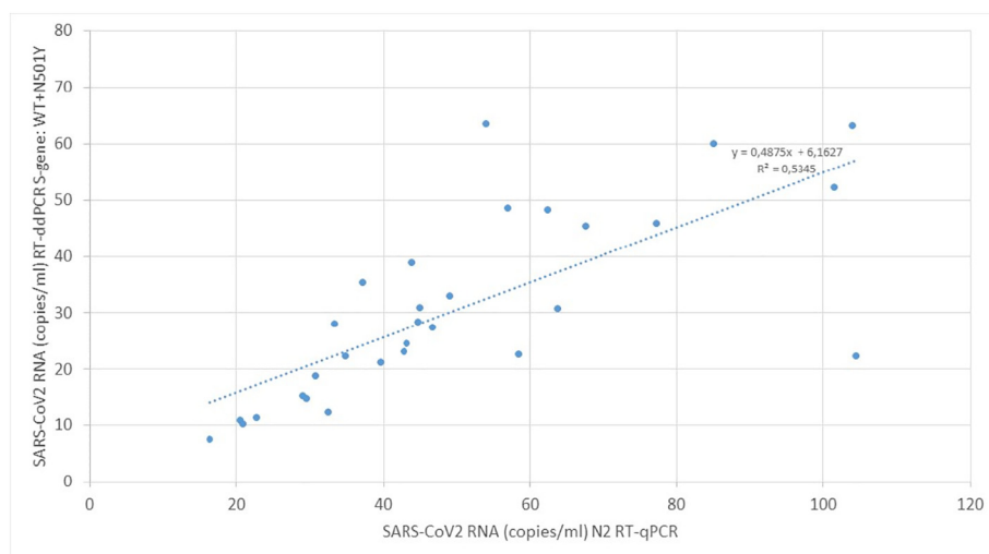
Fig. 6. Comparison of the wastewater concentrations of SARS-CoV-2 S-gene fragment, measured with RT-ddPCR, and the N2 gene fragment, measured with RT-qPCR. Wastewater samples from Amsterdam and Utrecht Nov 9 2020 – Mar 1 2021.
