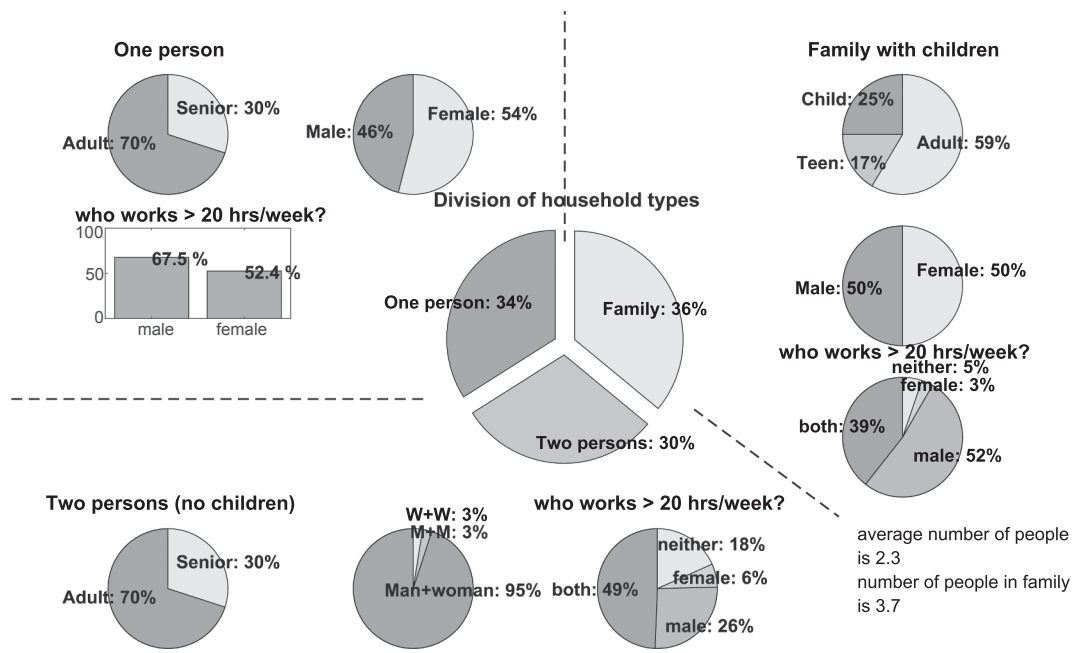
Fig. 2. SIMDEUM® household occupancy data used in Monte Carlo simulation (Blokker et al., 2010).
