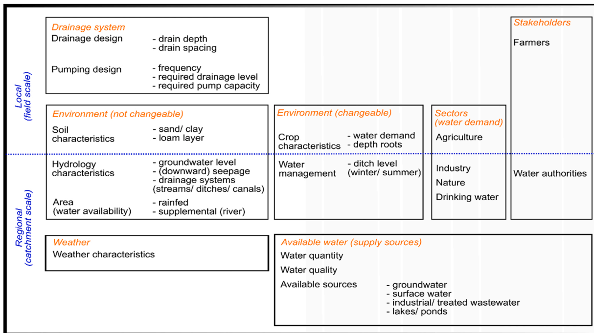
Fig. 7. Overview of local and regional scale components to take into account when implementing controlled drainage with subirrigation systems.
