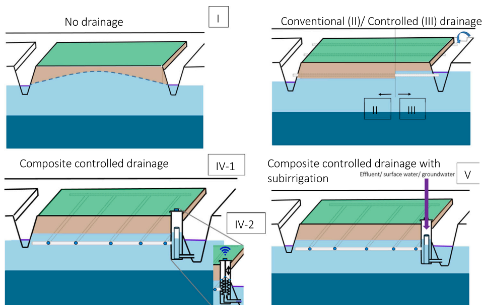
Fig. 3. Agricultural field without pipe drainage (I), with conventional drainage (II), with controlled drainage (III), with composite controlled drainage with a fixed weir (IV-1) or an online controlled weir structure (IV-2) and composite controlled drainage with subirrigation controlled by a fixed weir or online controlled weir structure (V).
