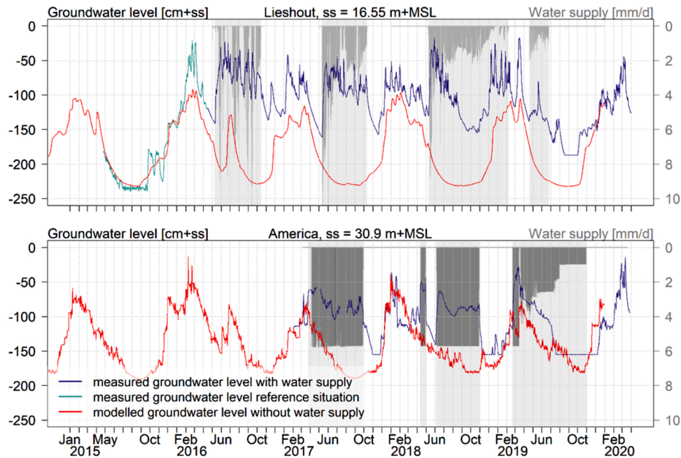
Fig. 4. Groundwater levels (cm+ soil surface, cm+ss) in two field experiments with a subirrigation-system: with water supply/subirrigation (blue, measured), reference situation (green, measured), and without water supply (red, modeled). The grey blocks represent the period of water supply (subirrigation), the dark grey blocks represent the amount of water supply. Figure adapted from de Wit et al. (2021a).
