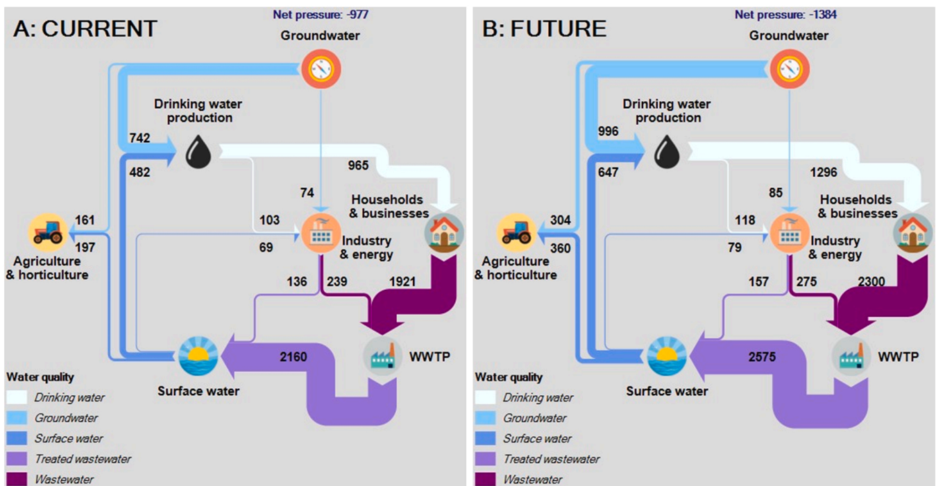
Fig. 8. Composite controlled drainage with subirrigation at field scale (part of ‘Agriculture and horticulture’) needs to fit in the regional water availability and demand for that water by multiple sectors. Left figure represents the anthropogenic water system of the Netherlands for the current situation, the right represents the anthropogenic water system of the Netherlands for the future (2050) situation. The flows and the net pressure on the groundwater system are given in million m 3 year -1 . Details about the flows are described in Pronk et al. (2021). Figures adapted from Pronk et al., 2021.
