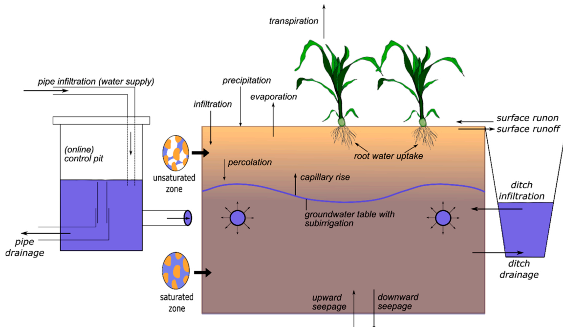
Fig. 5. The soil water column at field scale with the water balance components in the (un)saturated zone.
