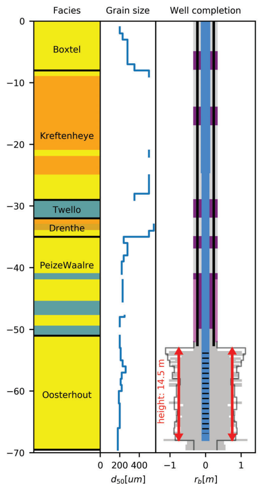
Figure 5. Drilling log and well completion of the EDGW at Espelo. The well radius is estimated based on both the volume of formation material removed from the borehole (gray line) and the volume of filter sand inserted in the well (gray polygon). Well radius scale is exaggerated relative to depth, displayed in m bgs.
