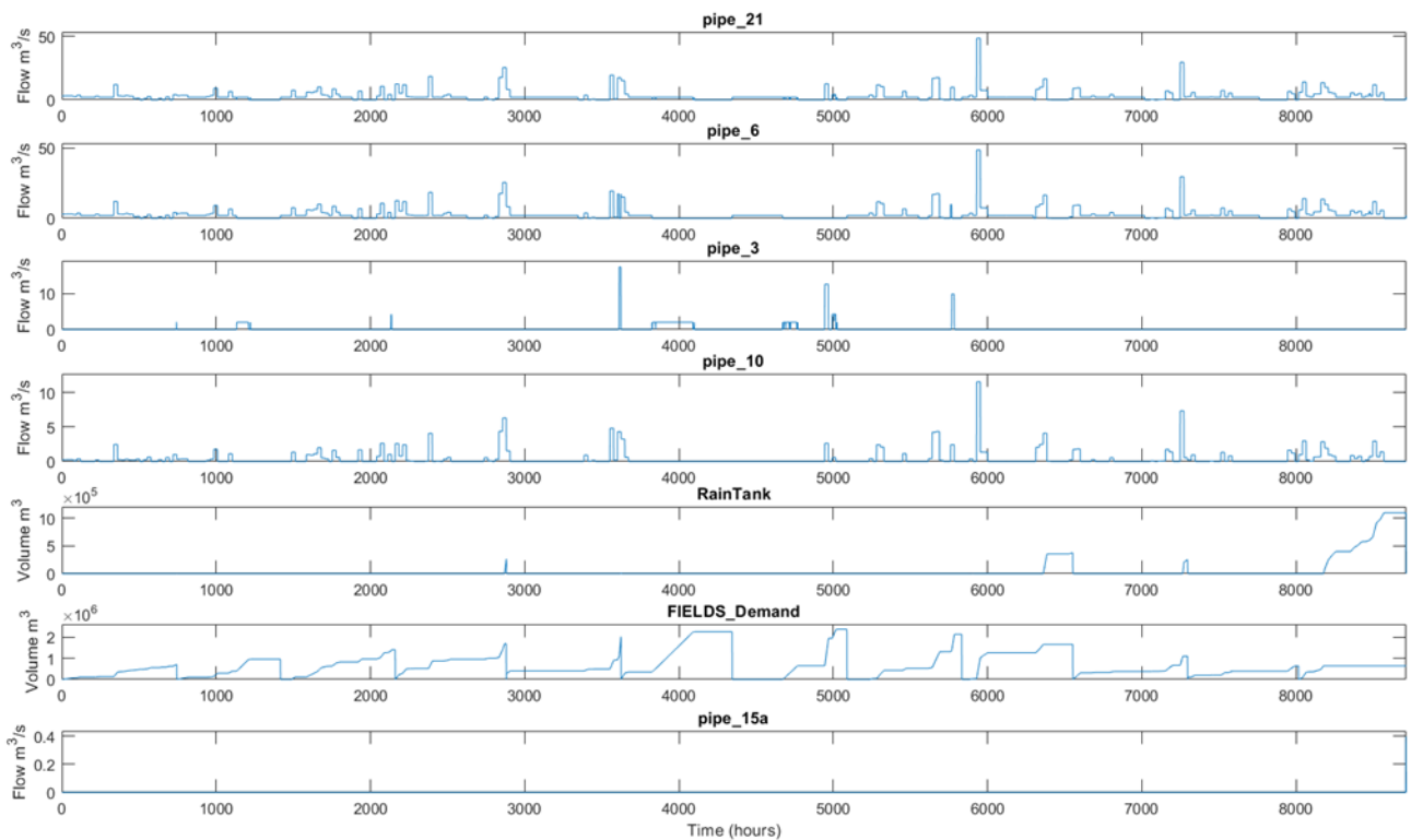
Figure 50 Different flows for Scenario 1, V2
