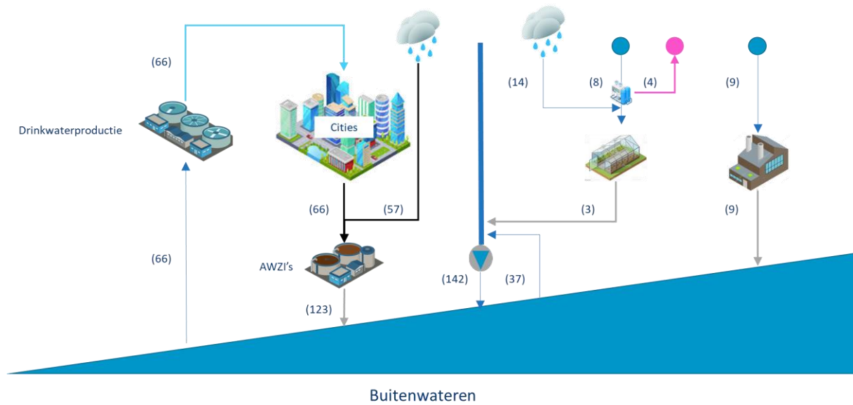
Figure 24 Hydraulic model of the base-line of Delfland demo case
