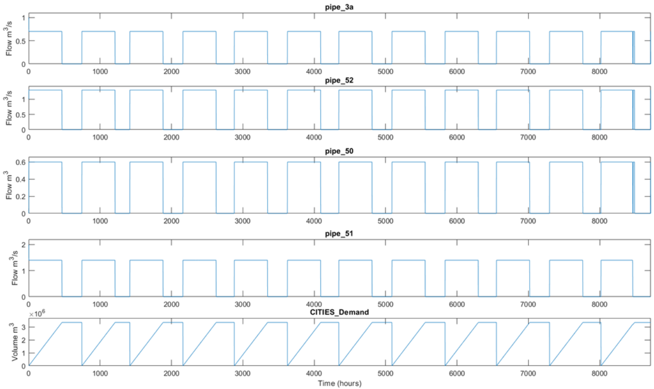
Figure 59 Different flows for Scenario 3, V3
