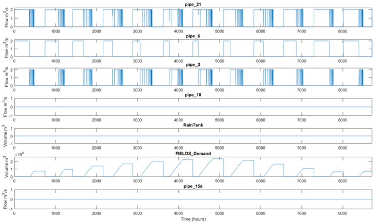
Figure 49 Different flows for Scenario 1, V1
