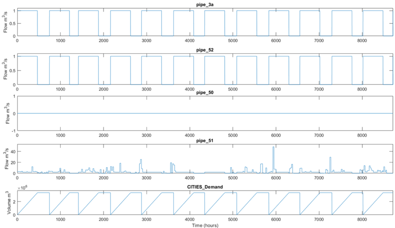
Figure 60 Different flows for Scenario 3, V4
