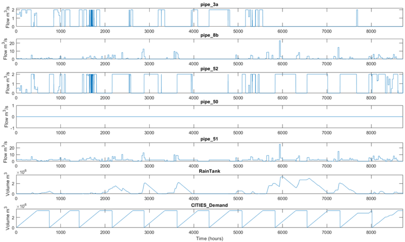
Figure 57 Different flows for Scenario 3, V1
