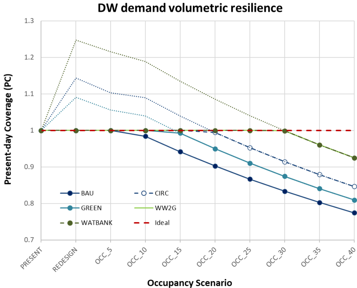
Figure 96 Resilience against increasing DW demands using the PC metric.
