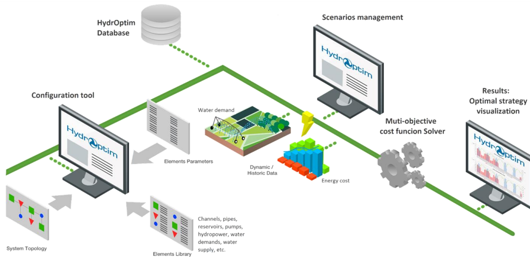
Figure 1 HydrOptim structure
