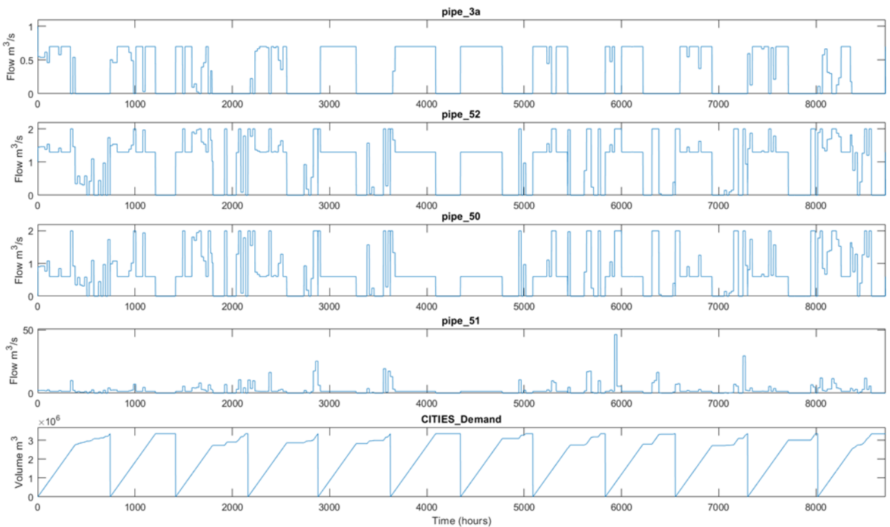
Figure 58 Different flows for Scenario 3, V2
