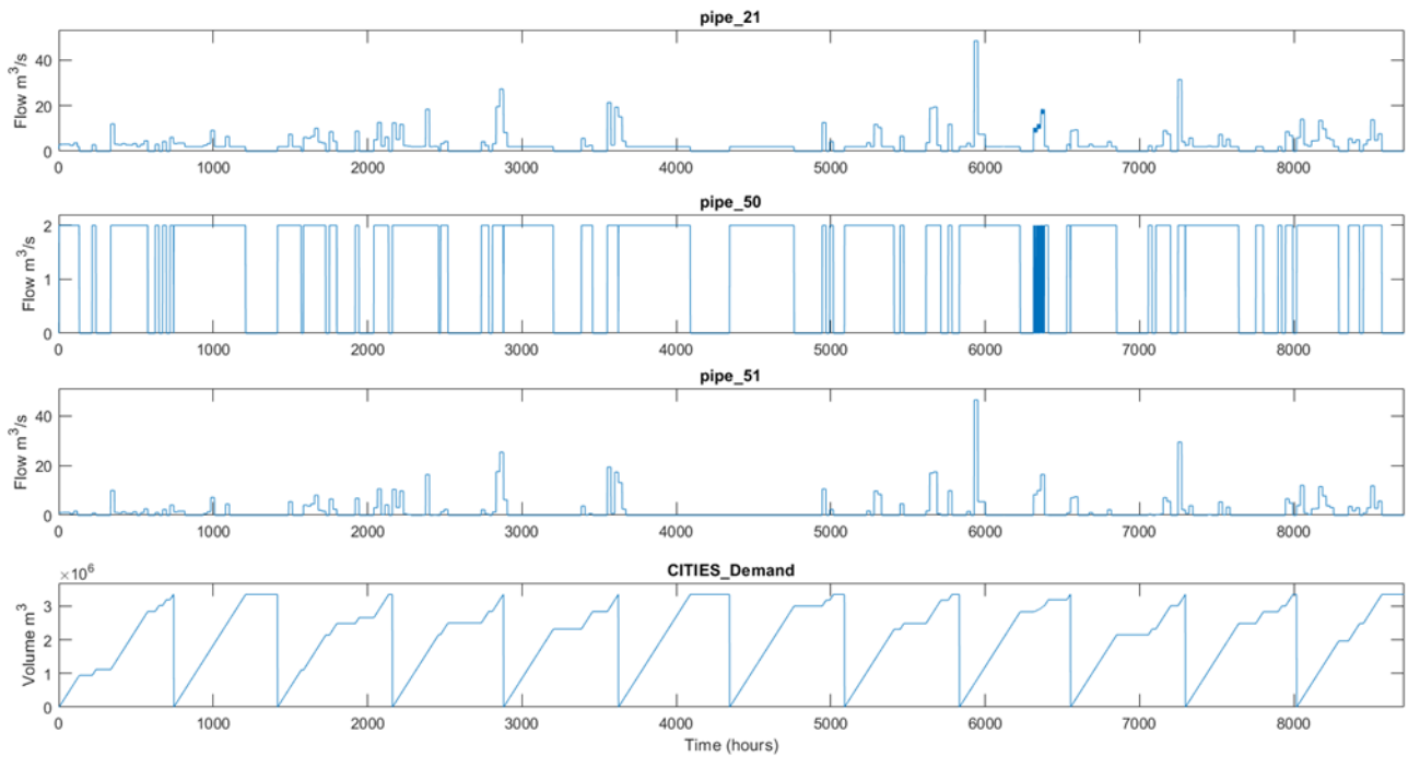
Figure 43 Flows in Pipe of WaterNode_3 for Scenario 3
