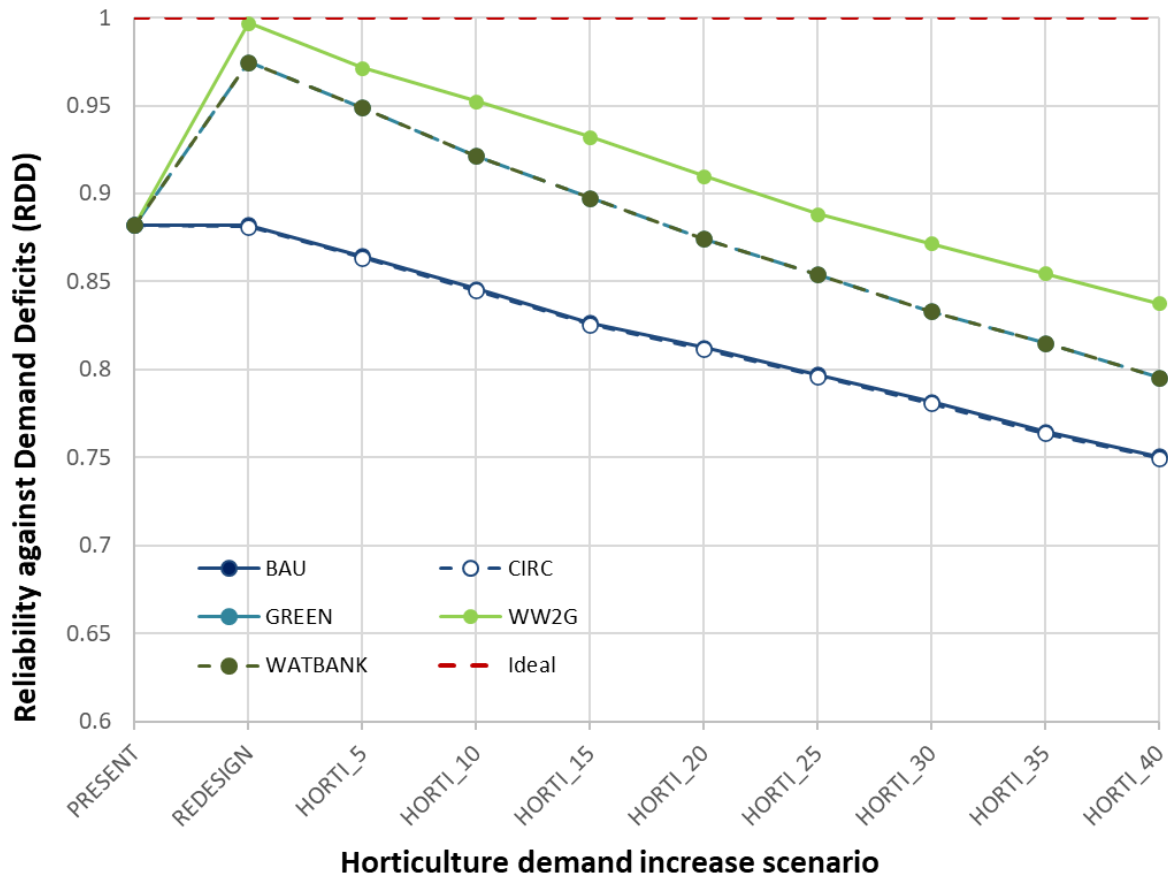
Figure 98 Resilience against increasing horticulture demands using the RDD metric.
