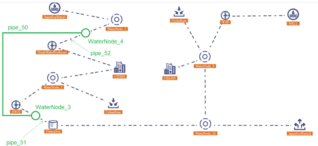
Figure 38 Changes in base line to implement Scenario 3
