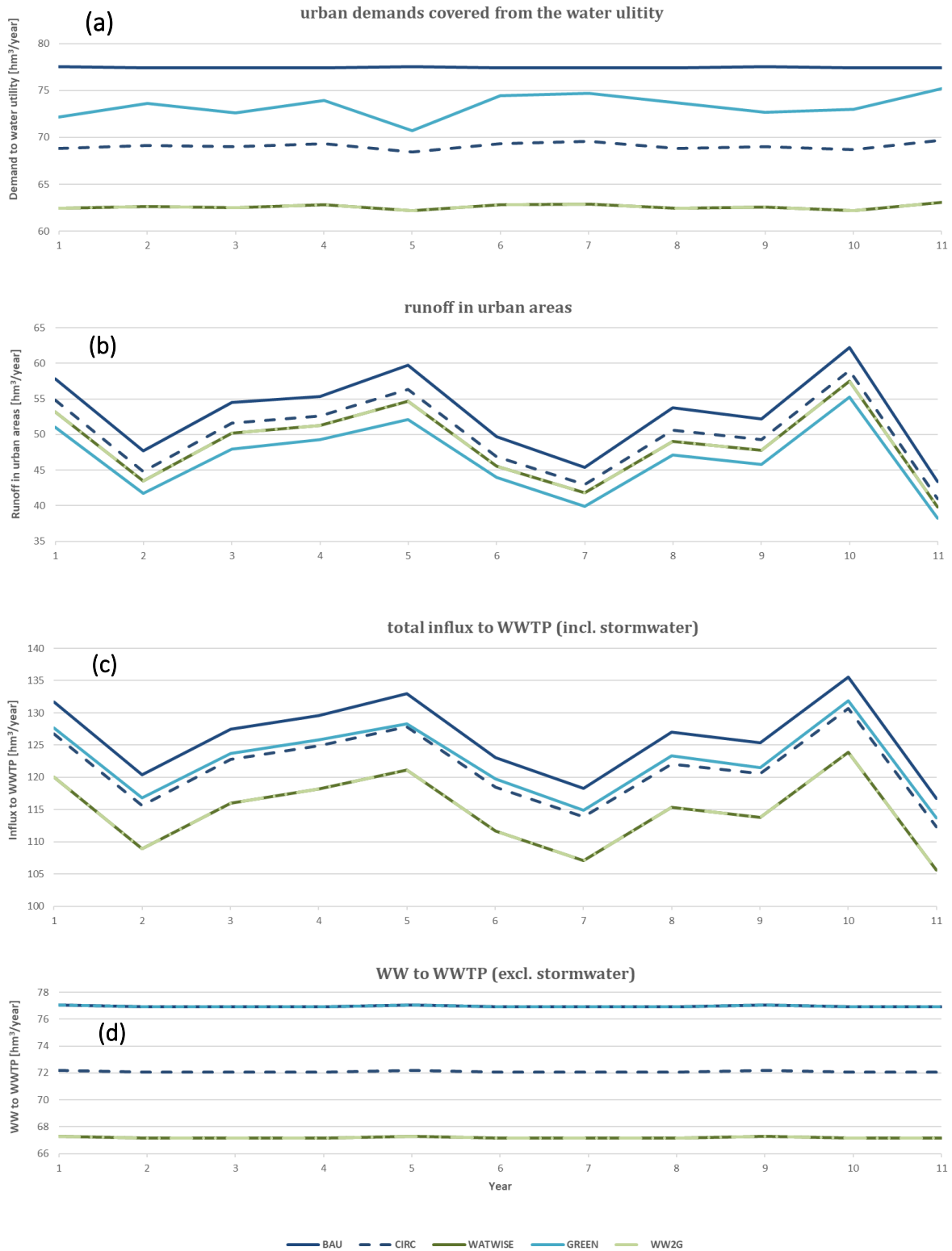
Figure 90 Results of redesign scenarios at the (inter-)annual scale.
