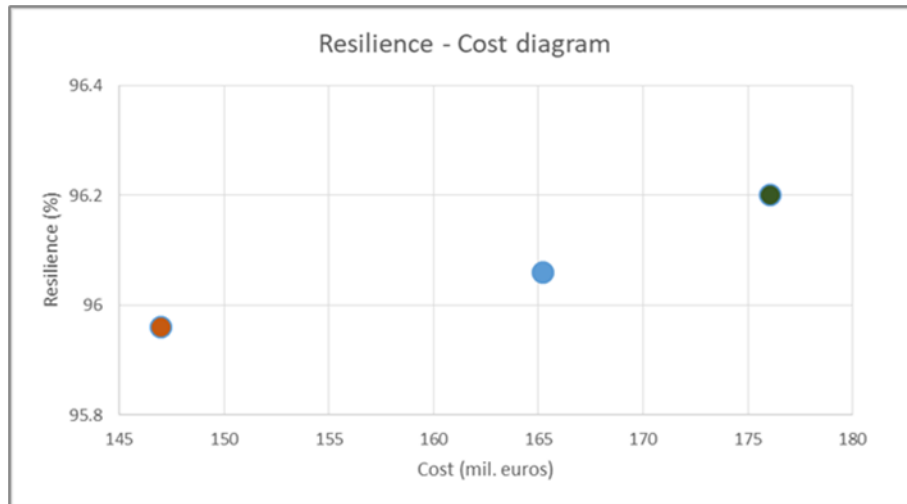
Figure 71 Resilience - Cost diagram
