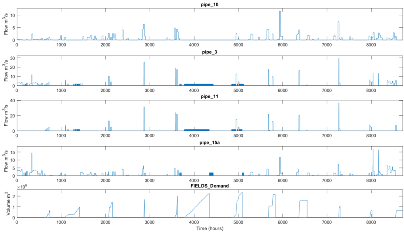
Figure 37 Flows in Pipe of WaterNode_9 for Scenario 1
