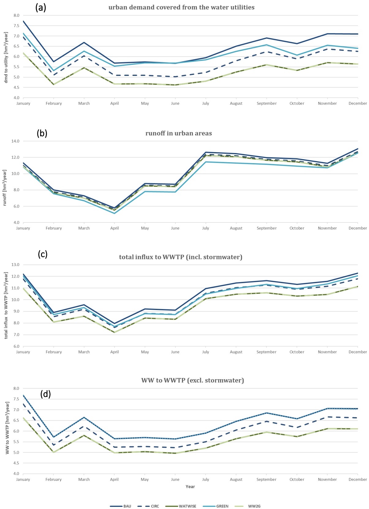
Figure 91 Results of redesign scenarios as average monthly flows.
