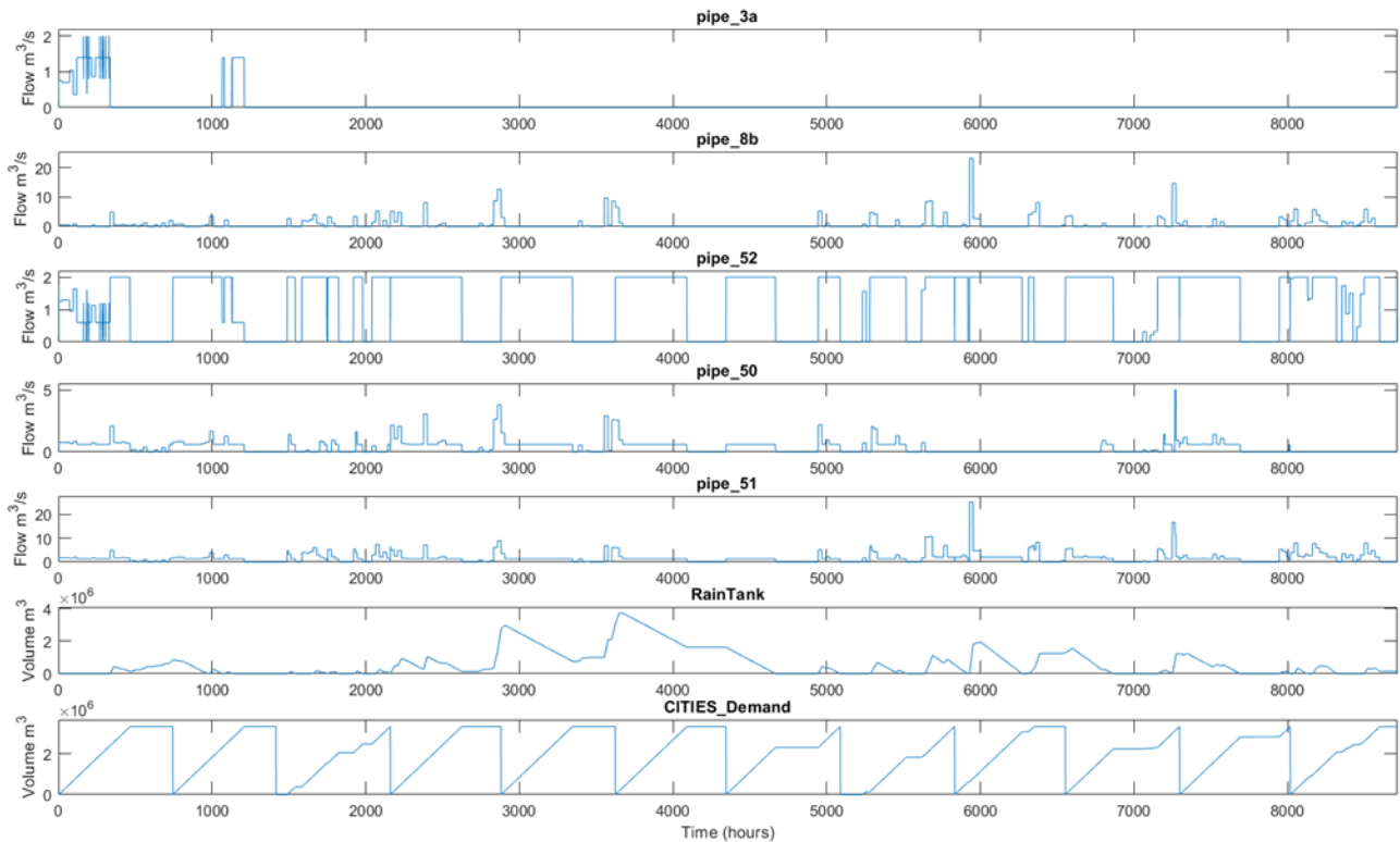
Figure 56 Different flows for Scenario 3, V0
