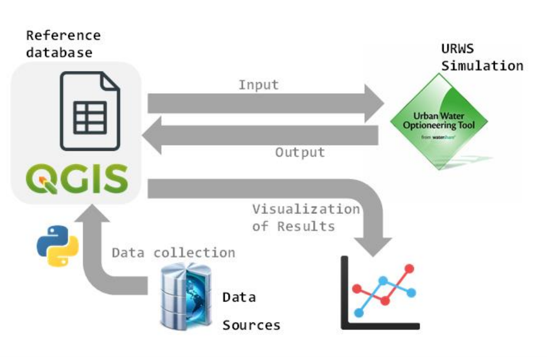
Figure 74 Schematic of the data preparation scheme that utilizes a reference database for model input and output.
