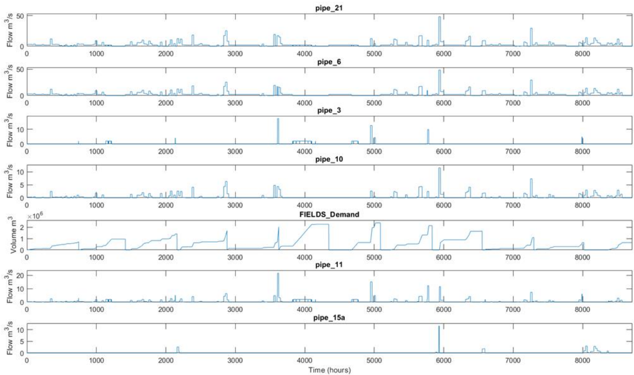
Figure 48 Different flows for Scenario 1, V0
