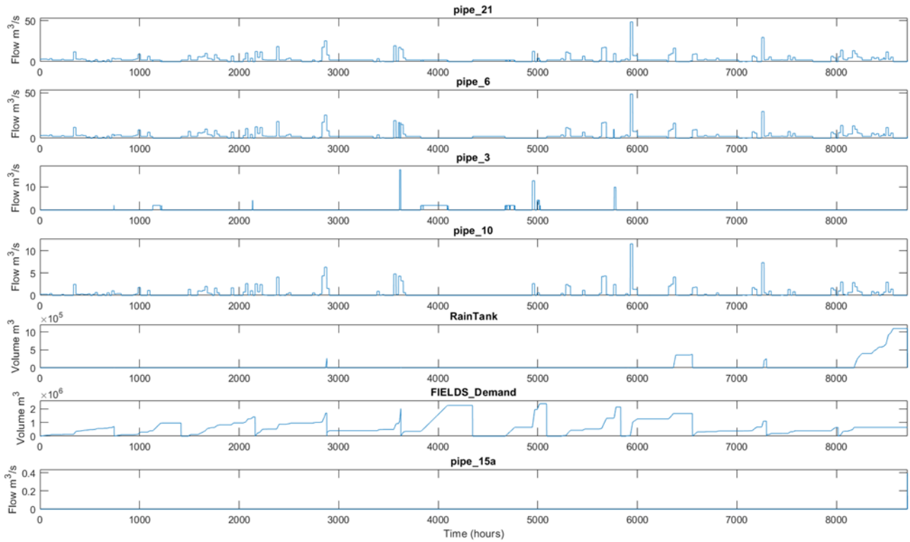
Figure 51 Different flows for Scenario 1, V3
