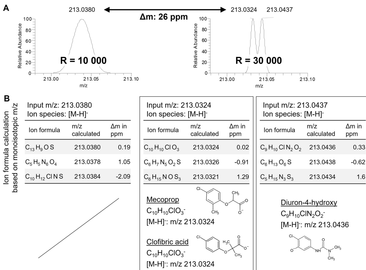
Fig. 6 Interplay between resolution (R) and mass accuracy exemplified by the two isomers mecoprop, clofibric acid and the isobar diuron-4-hydroxy. a Mass spectra for the isobaric ions acquired at a resolving power of 10,000 and 30,000. b Ion formula calculation based on the accurate monoisotopic mass and defining the ion species as [M - H] -
