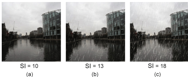
Fig. 4. Examples of synthetic rain images with the effect of increasing SI values: (a) SI = 10 ; (b) SI = 13 ; and (c) SI = 18 .
