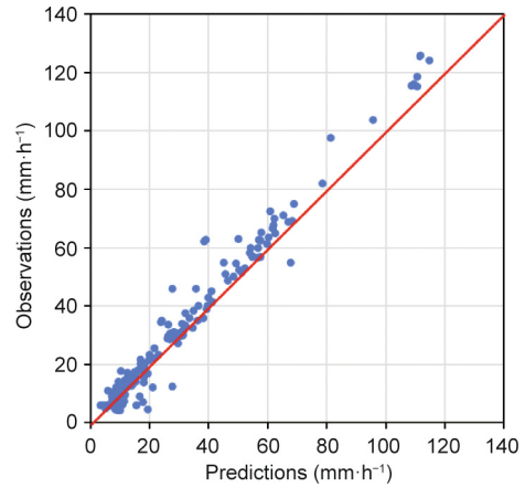
Fig. 9. Predictions vs observations based on the irCNN model applied to real rainfall images from smart phones (validation data).
