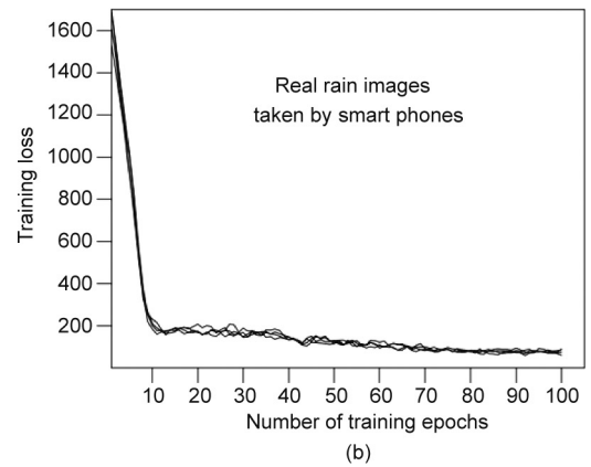
Fig. 8. Convergence trajectories of the proposed irCNN model runs: the convergence trajectories of the proposed model applied to (a) the synthetic dataset SD1 and (b) the real rainfall images from smart phones.
