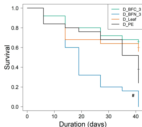
Figure 4. Survival of A. aquaticus during 7 weeks (42 days) on different food sources in Experiment D: Acer pseudoplatanus leaves (D_Leaf), biofilm cultured in drinking water from TP3 (D_BFC_3), natural biofilm on excavated PVC pipe (D_BFN_3) and PE without biofilm (D_PE). Survival of A. aquaticus is not significantly different from D_PE but does differ significantly from D_Leaf (#) (Cox Proportional Hazards model, comparison-wise error: p < 0.0125 ).
