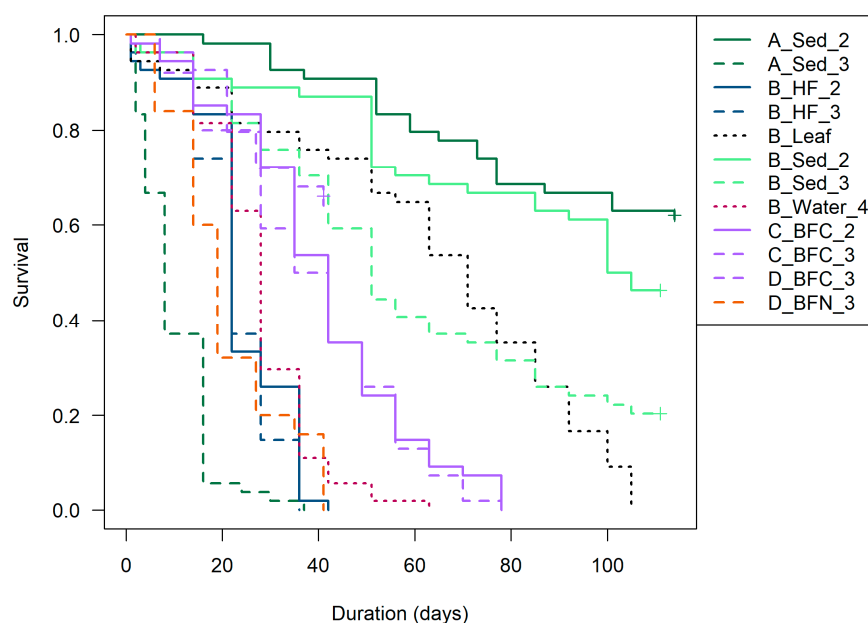
Figure 5. Survival of A. aquaticus on all tested food sources. For clarity, only one positive control (B_Leaf) and one negative control (B_Water_4) are included in the graph. +: experiment stopped. Information on statistically significant differences between conditions is given in Table 4.
