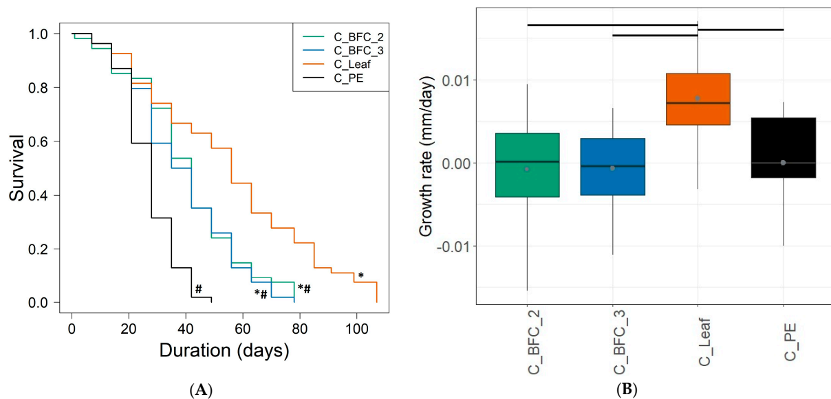
Figure 3. (A) Survival of A. aquaticus during 16 weeks (112 days) on different food sources in Experiment C: Acer pseudoplatanus leaves (C_Leaf), biofilm cultured in drinking water from TP2 (C_BFC_2) and TP3 (C_BFC_3) and PE without biofilm (C_PE). Survival of A. aquaticus is significantly different from C_PE (*) or from C_Leaf (#) (Cox Proportional Hazards model, comparison-wise error: p < 0.0125 ). (B) Growth rate of A. aquaticus between days 0 and 28. Horizontal black bars indicate significantly different growth rates (Kruskal–Wallis test with Dunn’s test and Bonferroni post hoc test, p < 0.05 ).
