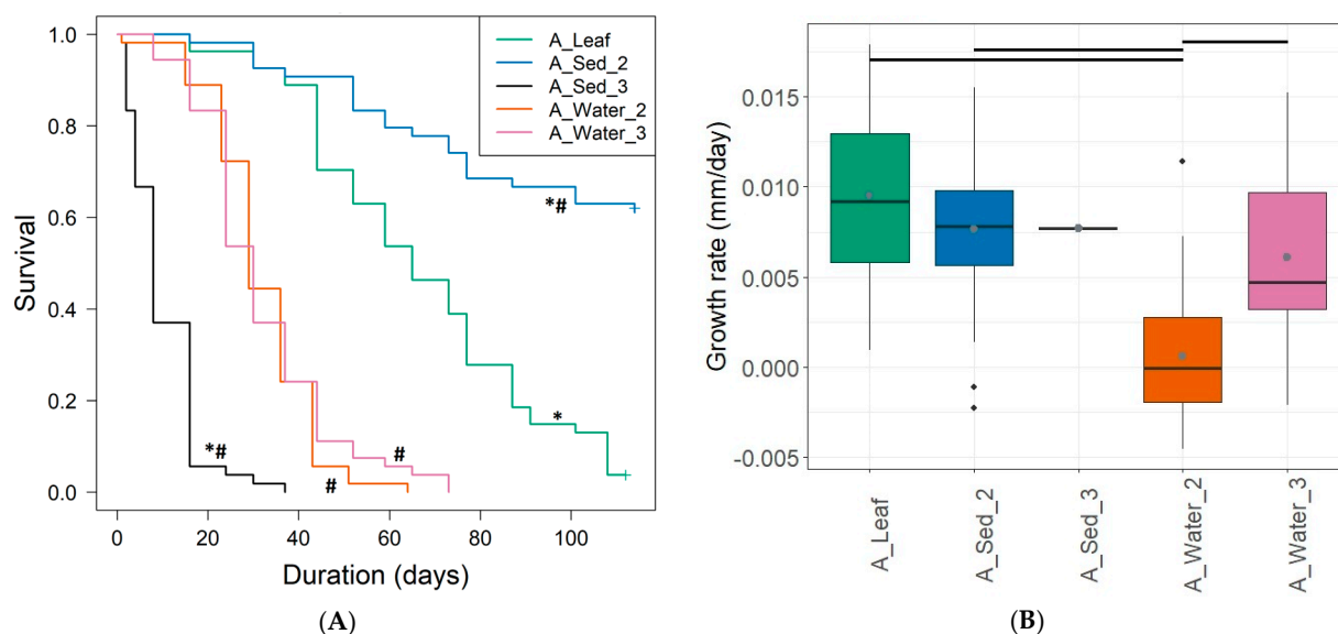
Figure 1. (A) Survival of A. aquaticus during 16 weeks (112 days) on different food sources in Experiment A: Acer pseudoplatanus leaves (A_Leaf), sediment from DWDS2 (A_Sed_2) and DWDS3 (A_Sed_3) and water from TP2 (A_Water_2) and TP3 (A_Water_3). * Survival of A. aquaticus is significantly different from A_Water_2 (*) or from A_Leaf (#) (Cox Proportional Hazards model, comparison-wise error: p < 0.01 ). (B) The growth rate of A. aquaticus between Days 0 and 28. The growth rate of A_Sed_3 was determined for only a few specimens due to the high mortality rate. Horizontal black bars indicate significantly different growth rates between the two conditions at which the bar starts or stops, e.g., A_Leaf vs. A_Water_2 (Kruskal–Wallis test with Dunn’s test and Bonferroni post hoc test, p < 0.05 ).
