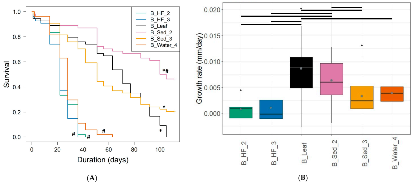
Figure 2. (A) Survival of A. aquaticus during 16 weeks (112 days) on different food sources in Experiment B: Acer pseudoplatanus leaves (B_Leaf), sediment from DWDS2 (B_Sed_2) and DWDS3 (B_Sed_3), water from DWDS4 (B_Water_4) and concentrate from DWDS2 (B_HF_2) and DWDS3 (B_HF_3). Survival of A. aquaticus is significantly different from B_Water_4 (*) or from B_Leaf (#) (Cox Proportional Hazards model, p < 0.05 ). (B) Growth rate of A. aquaticus between Days 0 and 28. Horizontal black bars indicate significantly different growth rates (Kruskal–Wallis test with Dunn’s test and Bonferroni post hoc test, p < 0.05 ).
