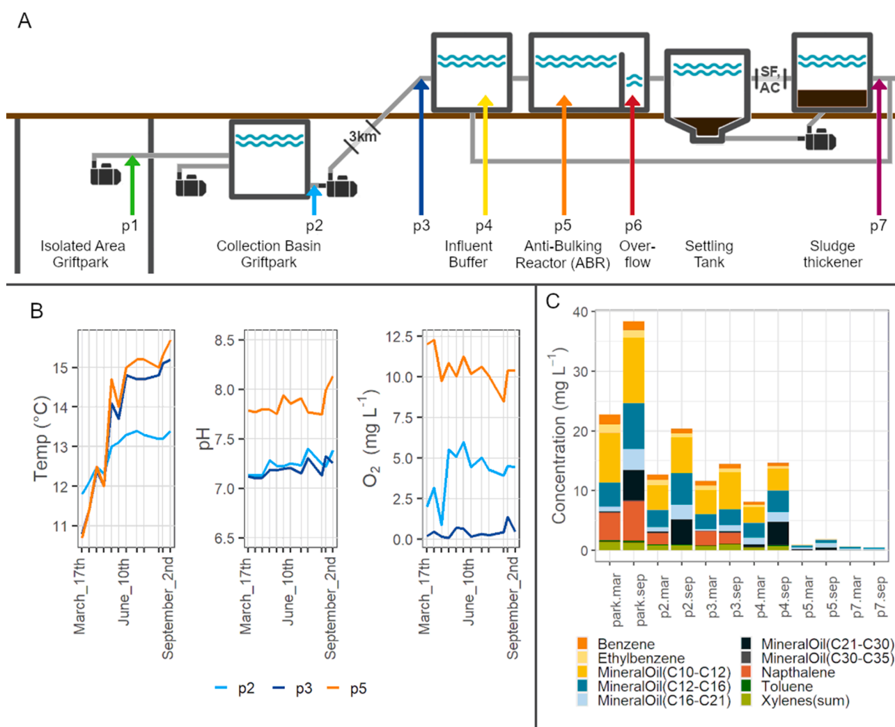
Figure 2. A. Schematic overview of the Griftpark Groundwater Treatment Pipeline. Seven sampled points are indicated with colored arrows. B. Temperature, pH, and oxygen content of the pipelines between March and September 2016 (data collected by municipality). C. Total pollutant concentration in the park groundwater and at sampling points p2, p3, p4, p5, and p7 on the 18 th of March, and the 16 th of September 2016, as provided by the municipality.
