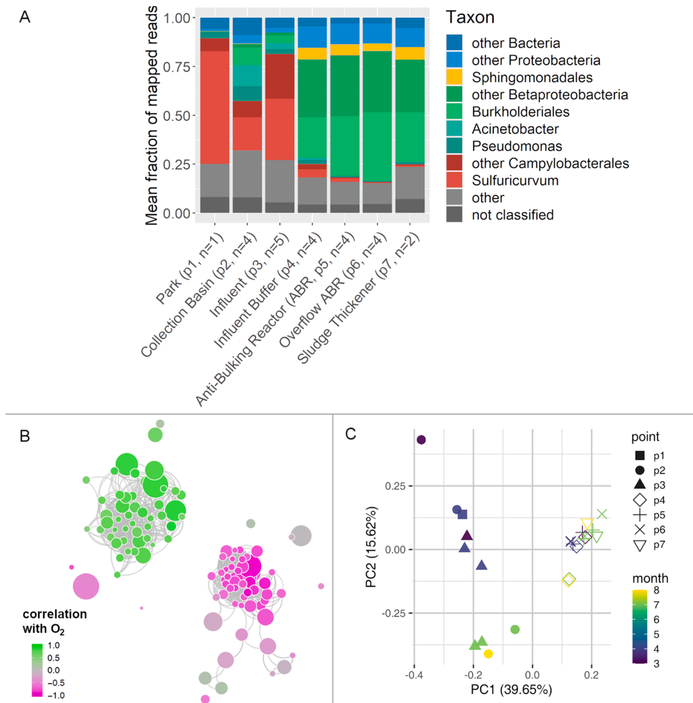
Figure 3. The microorganisms in the treatment pipeline cluster into two distinct groups. A. Relative abundance of the most abundant taxa in the treatment pipeline in mean fraction of mapped reads belonging to that taxon. B. Co-response network of the microbial communities. Nodes represent organisms with a relative abundance of at least 0.1% in a minimum of two samples (n=94). Edges connect organisms that have a Spearman correlation \geq 0.75 . The nodes are colored according to the Spearman correlation of the taxa with oxygen concentration. The full network with organism annotation can be found in Supplementary Figure S3. Similar plots for other environmental variables including oxygen, pH, and pollutant concentrations are shown in Supplementary Figures S4-S18. C. Principal component analysis based on relative abundance of taxa in all 24 samples showing high similarity between plant-side communities (p4-p7) and structuring of the park-side communities by date along PC2.
