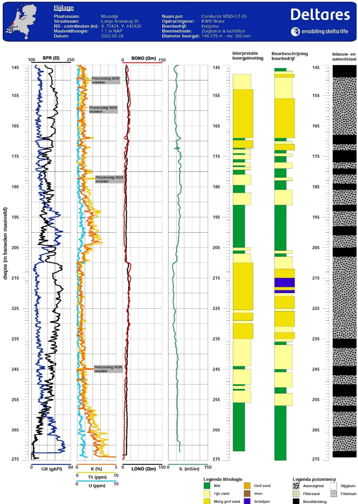
Figure 26 Lithological interpretation and well completion information from 145 to 275m depth, by Deltares based on the logging data and cuttings description.
