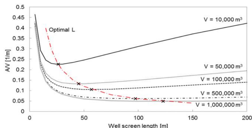
Figure 7. Optimum well screen length for given injection volumes, to minimise conduction losses (Bloemendal and Hartog, 2018).
