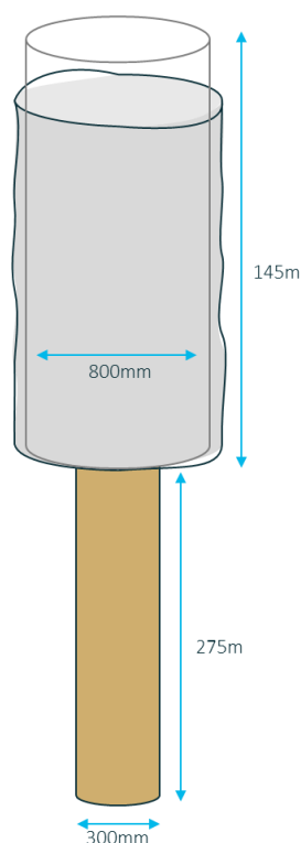
Schematic representation of the deepening drilling as carried out at the TRIAS Westland site.
