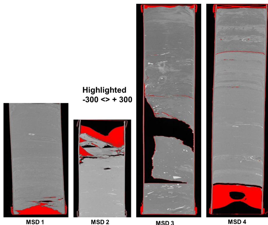
Figure 24 CT-scan with red highlight on zone with CT-scan value of -300 to 300, indicating the volume that is filled with density of water/paraffin. MSD1 was only half filled, empty top part is not scanned. Dark = low density, white = high density.
